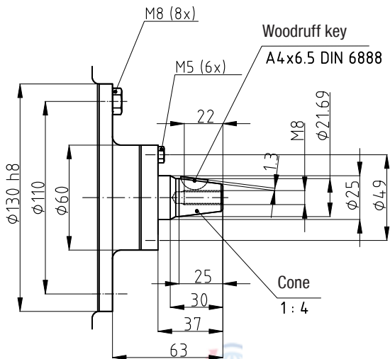
Fig. 26 Dimensions in mm Dimensions for view X see page 32
