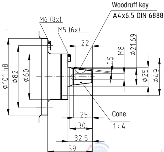
Fig. 37 Dimensions in mm Dimensions for view X see page 40
